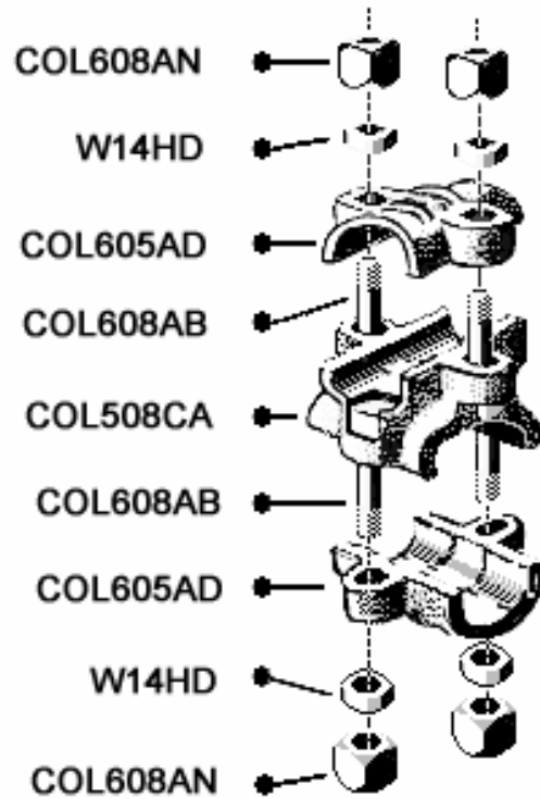
COL608CAX Universal Clamp Assembly
