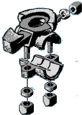
COL606X Swing Dump Clamp
