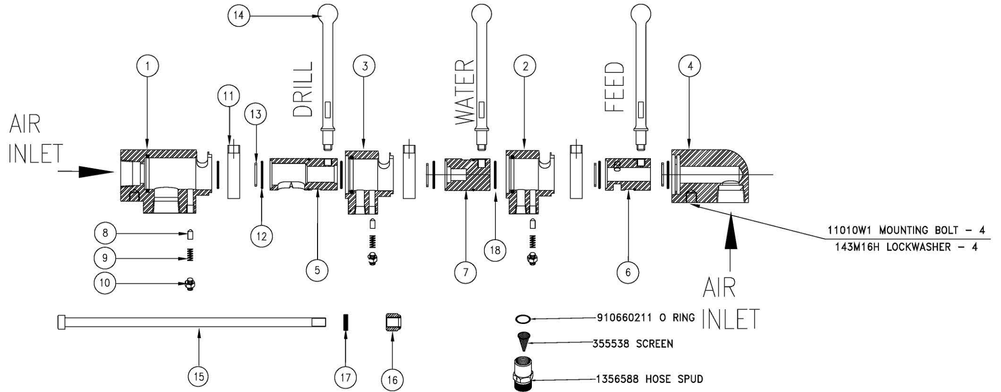
JC45 FILTER ASSEMBLY
